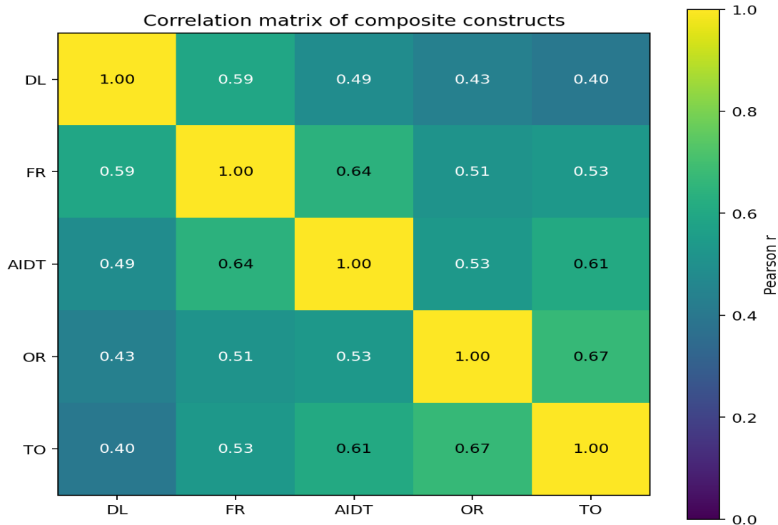
Figure 2. Pearson correlation matrix (synthetic data).
