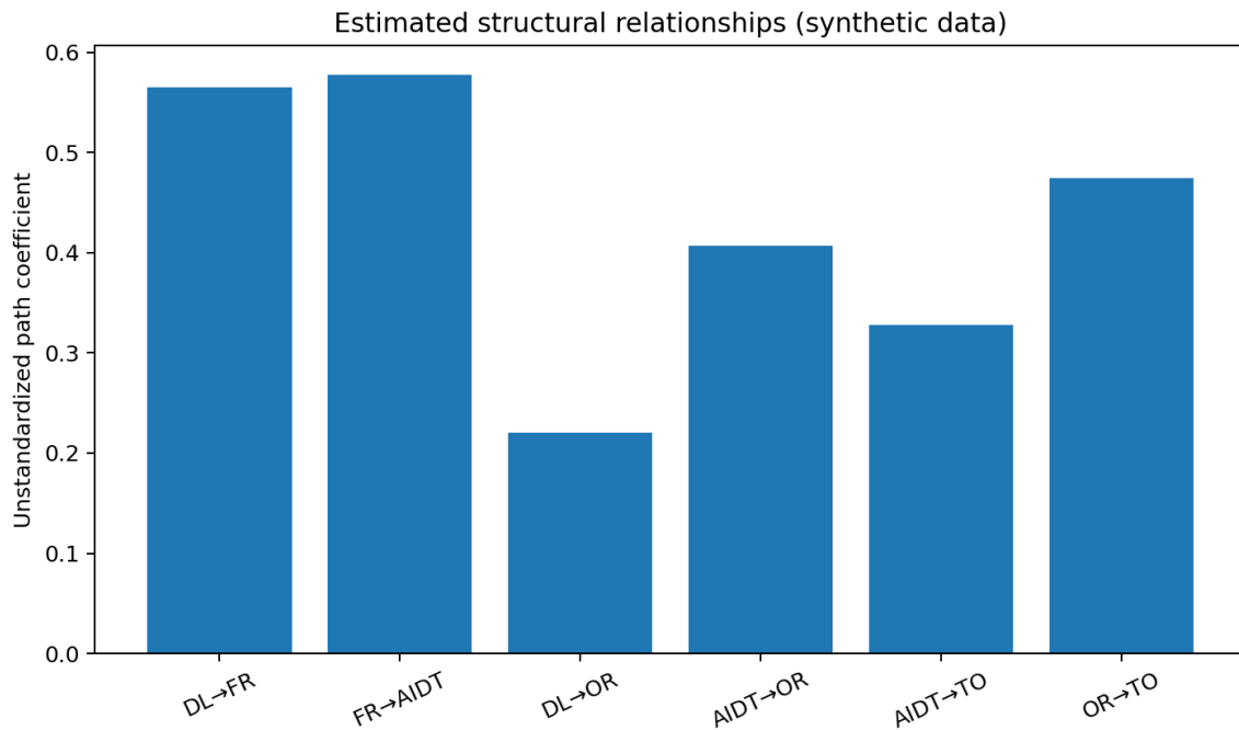
Figure 3. Estimated direct-effect coefficients (synthetic data).
