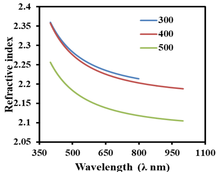
Figure 3.3: Validation of refractive index by Reflectometer (thickness 300, 400 and 500 nm)
